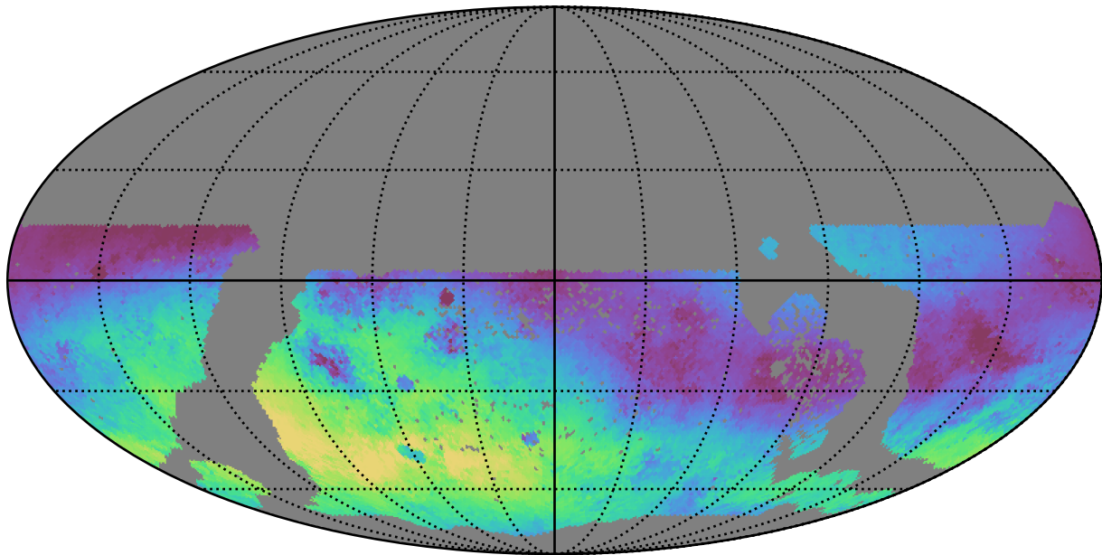
too_100_4v3.4_10yrs WFD g band: Median skyBrightness
