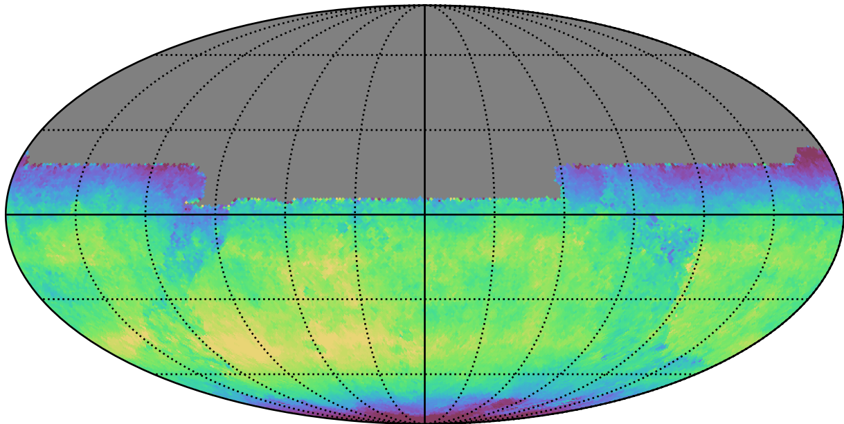
too_100_4v3.4_10yrs All sky y band: Median skyBrightness
