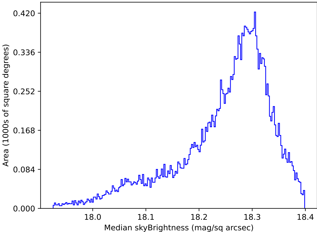
too_100_4v3.4_10yrs All sky y band: Median skyBrightness
