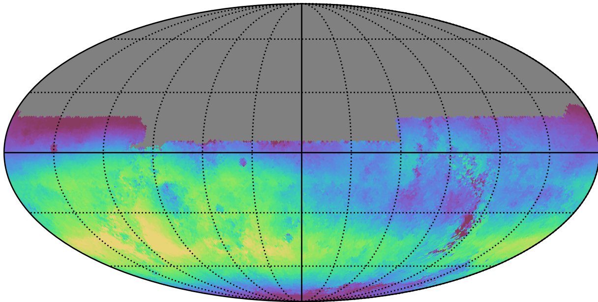
too_100_4v3.4_10yrs All sky u band: Median skyBrightness
