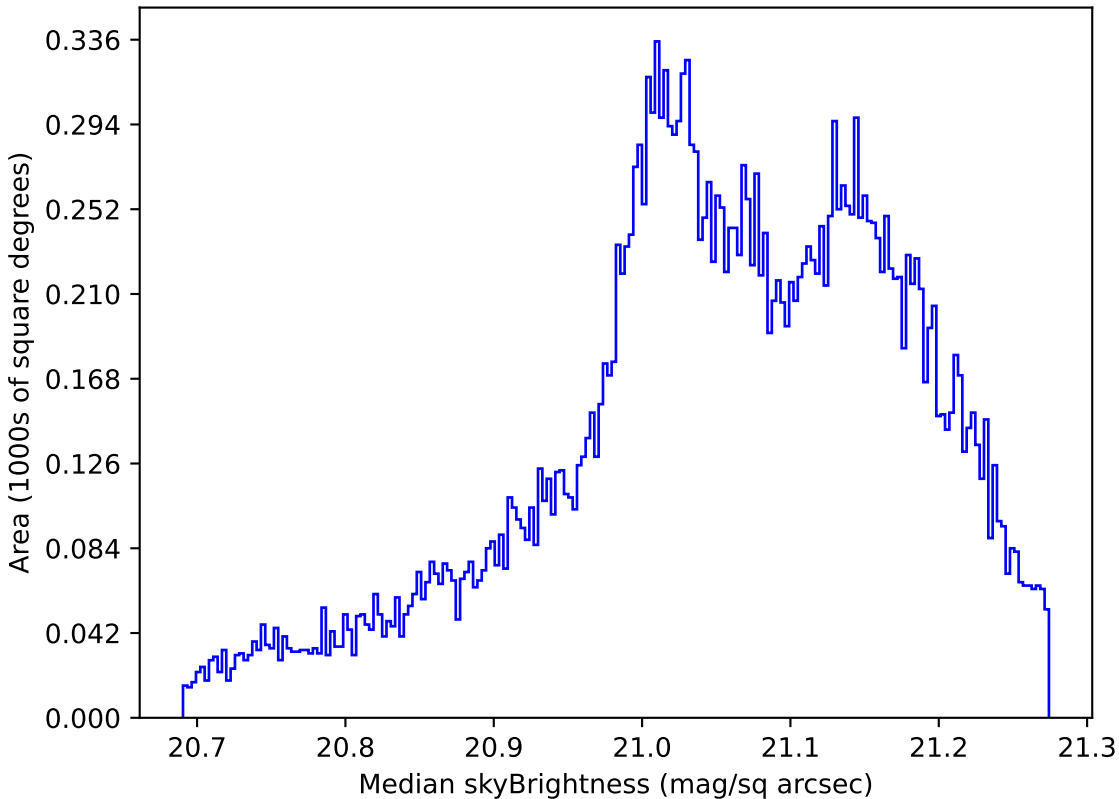
too_100_4v3.4_10yrs All sky r band: Median skyBrightness
