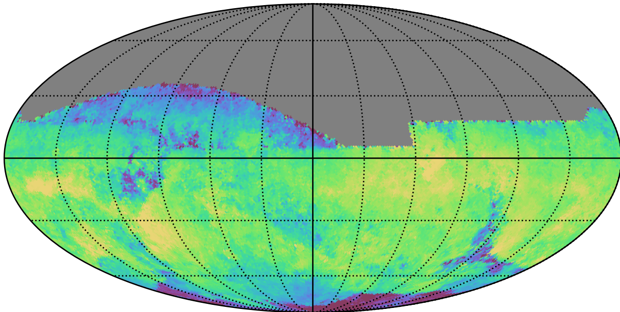
too_100_4v3.4_10yrs All sky i band: Median skyBrightness
