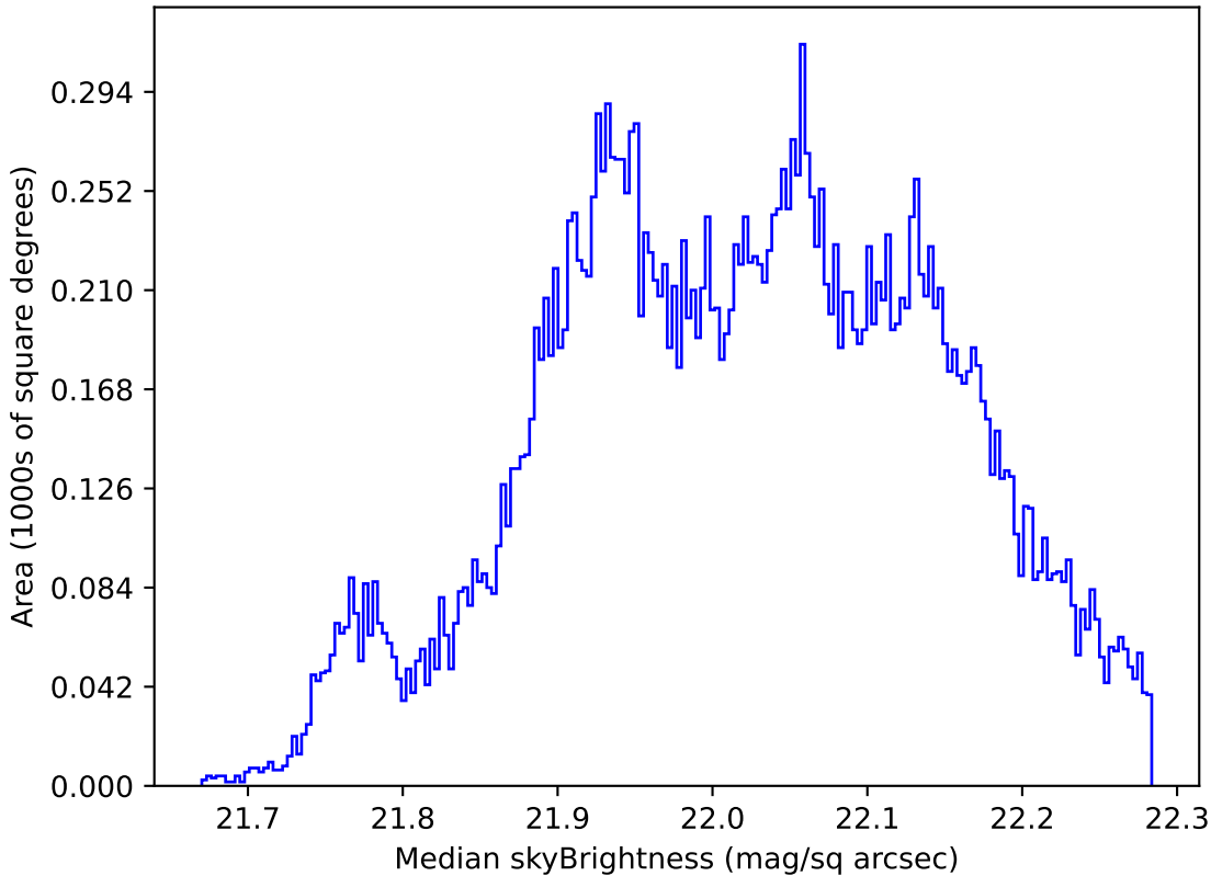
too_100_4v3.4_10yrs All sky g band: Median skyBrightness
