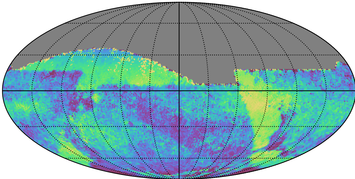
too_100_4v3.4_10yrs All sky all bands: Median skyBrightness
