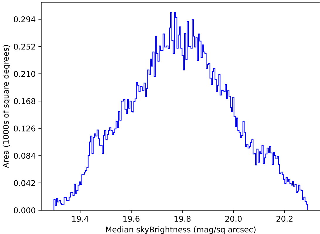
too_100_4v3.4_10yrs All sky all bands: Median skyBrightness
