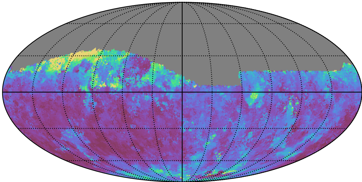
too_100_4v3.4_10yrs Yr 1 z band: Median seeingGeom
