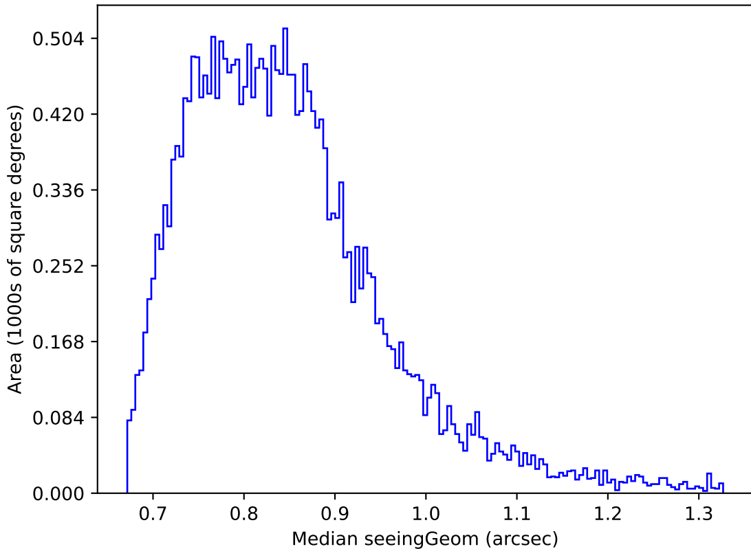
too_100_4v3.4_10yrs Yr 1 z band: Median seeingGeom
