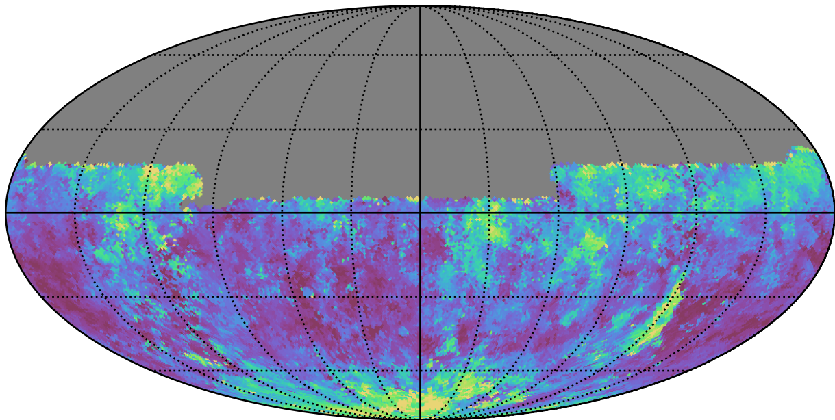
too_100_4v3.4_10yrs Yr 1 y band: Median seeingGeom
