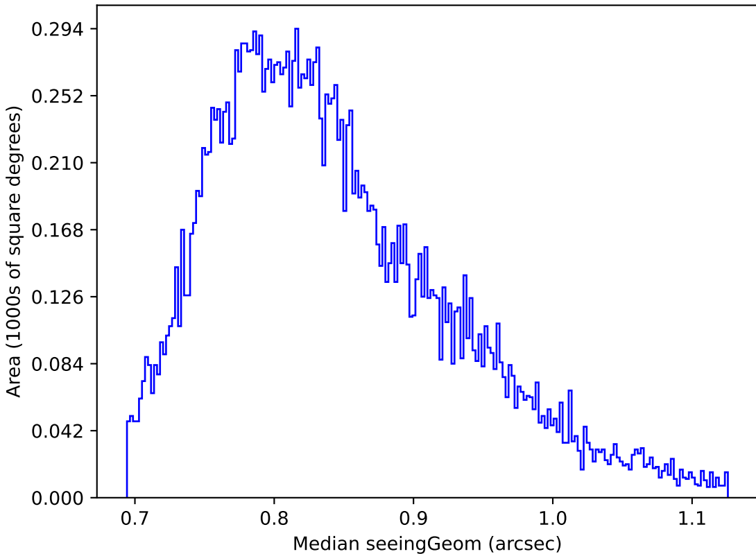
too_100_4v3.4_10yrs Yr 1 y band: Median seeingGeom
