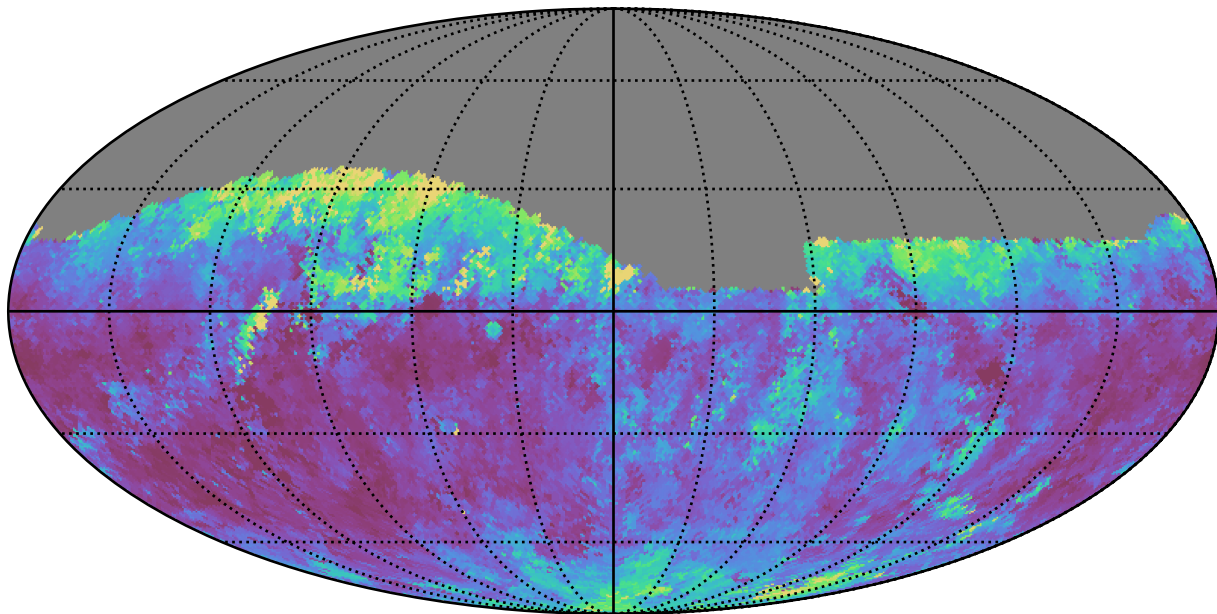
too_100_4v3.4_10yrs Yr 1 r band: Median seeingGeom
