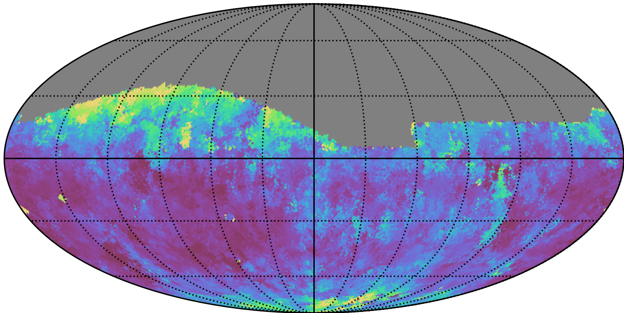
too_100_4v3.4_10yrs Yr 1 i band: Median seeingGeom
