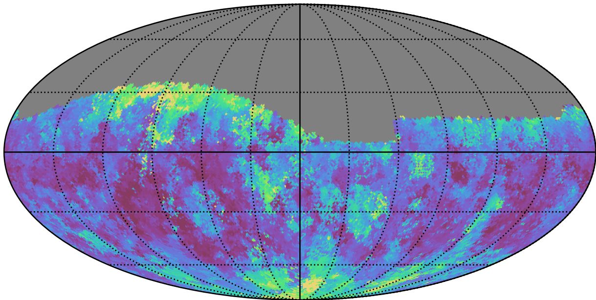
too_100_4v3.4_10yrs Yr 1 g band: Median seeingGeom
