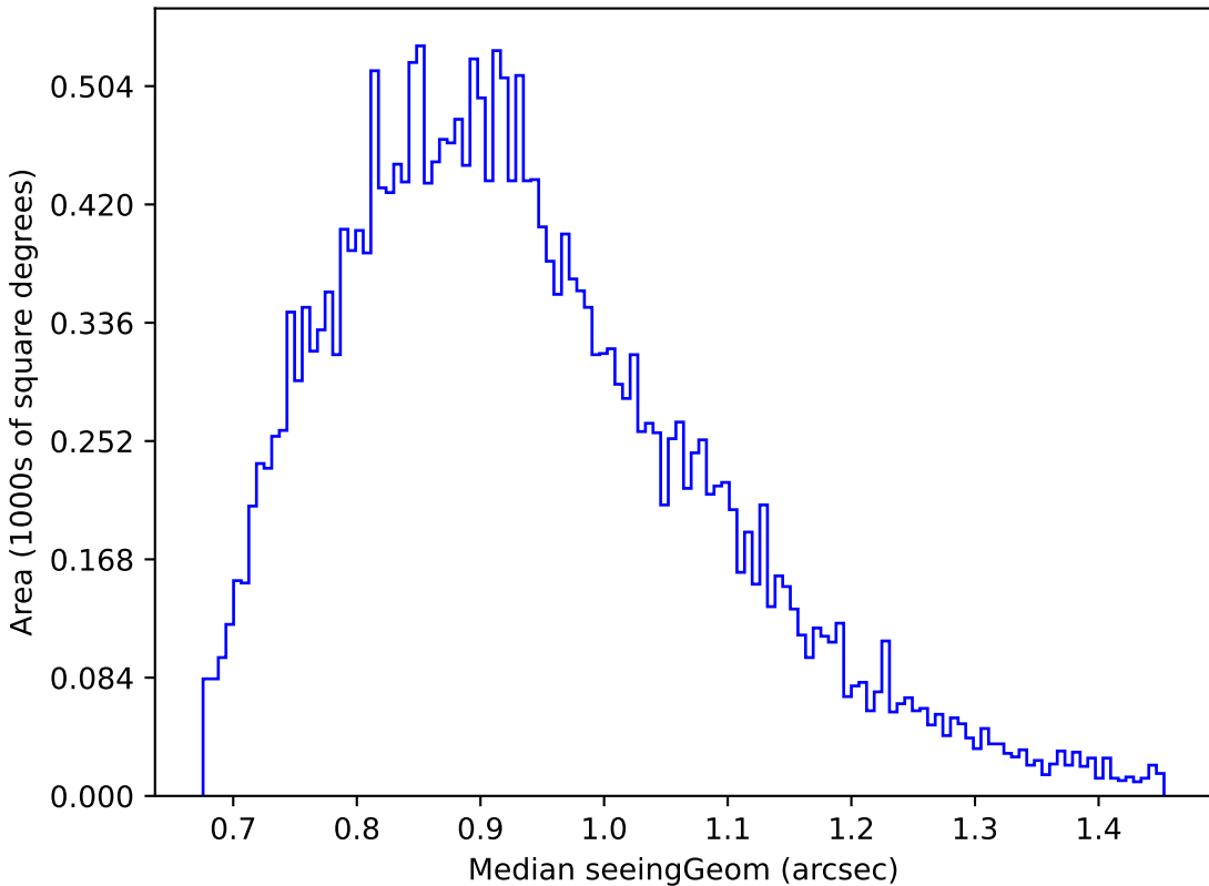
too_100_4v3.4_10yrs Yr 1 g band: Median seeingGeom
