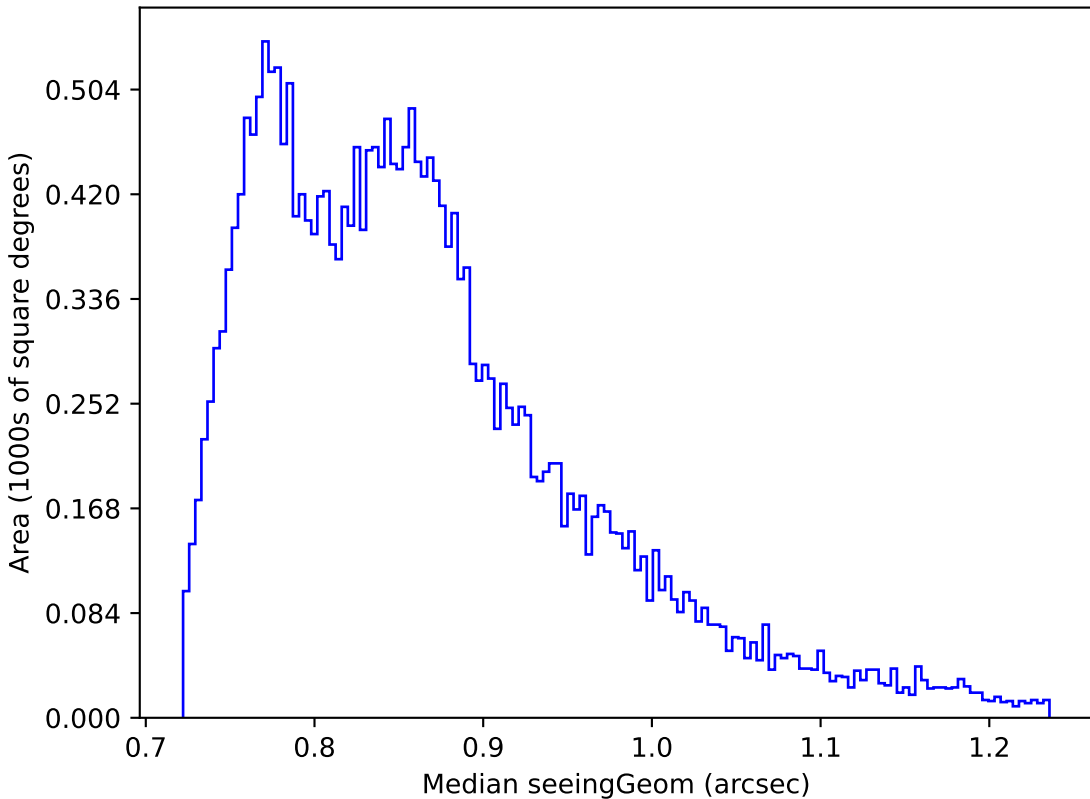
too_100_4v3.4_10yrs Yr 1 all bands: Median seeingGeom
