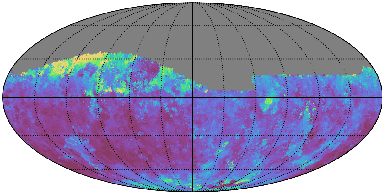
too_100_4v3.4_10yrs Yr 1 z band: Median seeingEff
