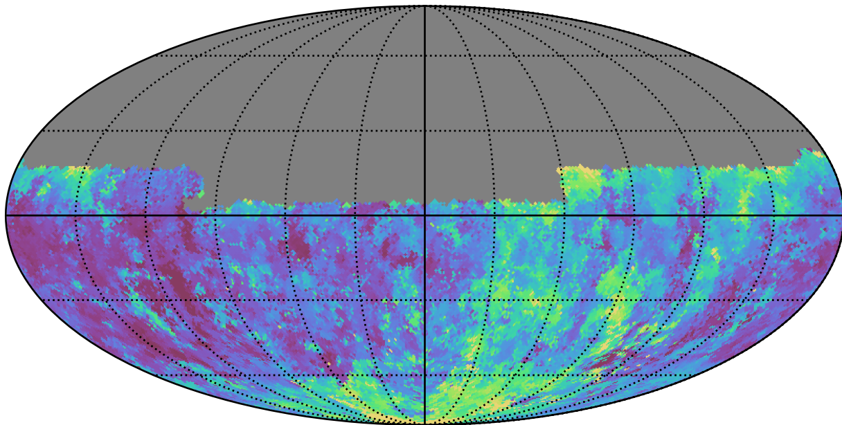
too_100_4v3.4_10yrs Yr 1 u band: Median seeingEff
