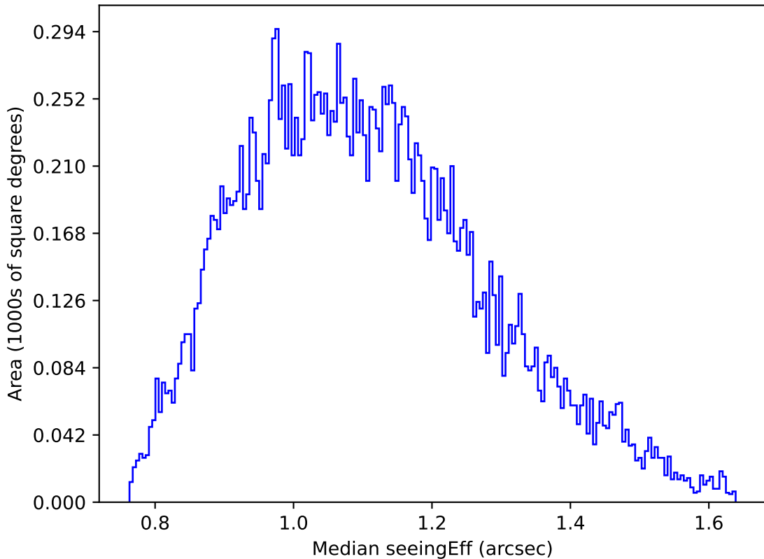
too_100_4v3.4_10yrs Yr 1 u band: Median seeingEff
