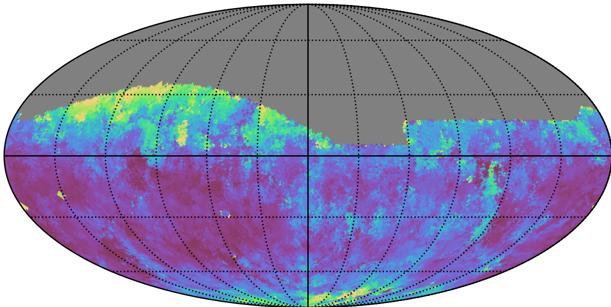
too_100_4v3.4_10yrs Yr 1 i band: Median seeingEff
