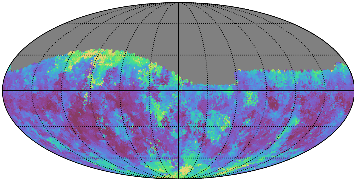
too_100_4v3.4_10yrs Yr 1 g band: Median seeingEff
