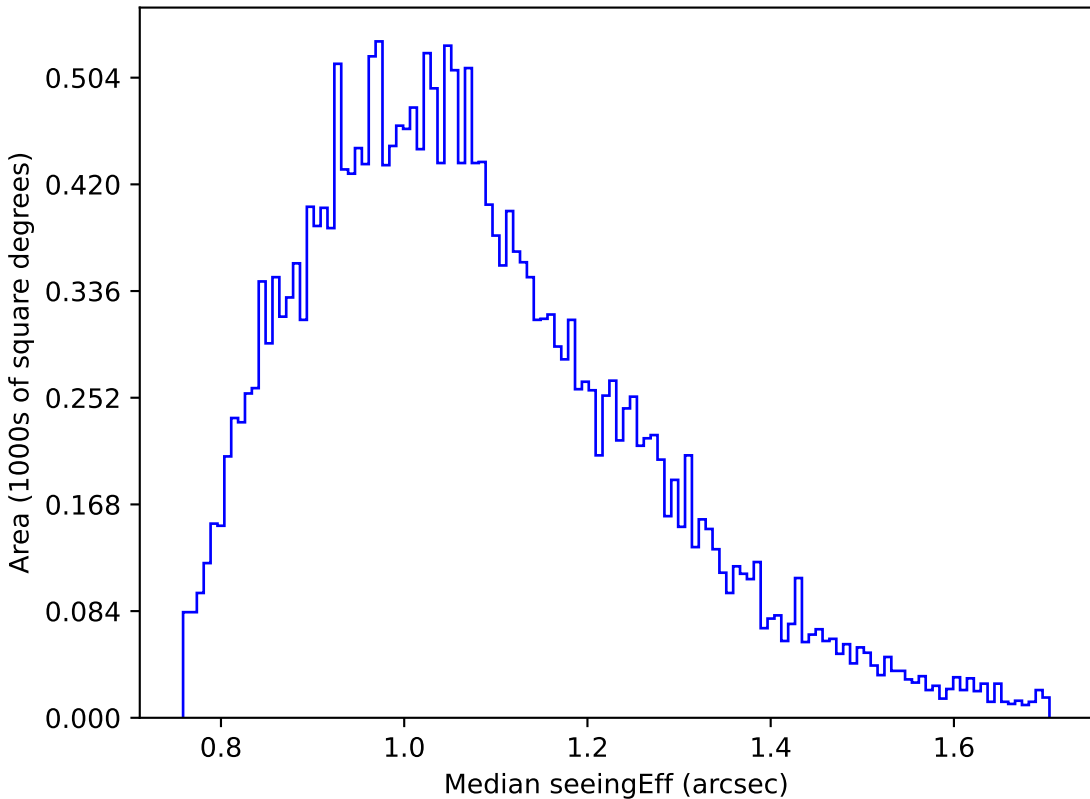
too_100_4v3.4_10yrs Yr 1 g band: Median seeingEff
