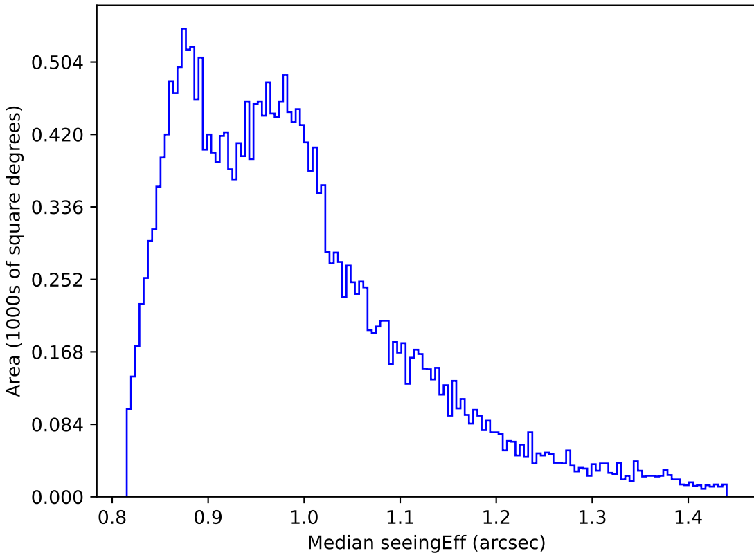
too_100_4v3.4_10yrs Yr 1 all bands: Median seeingEff
