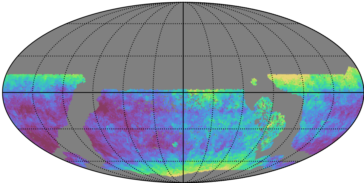
too_100_4v3.4_10yrs WFD y band: Median seeingEff
