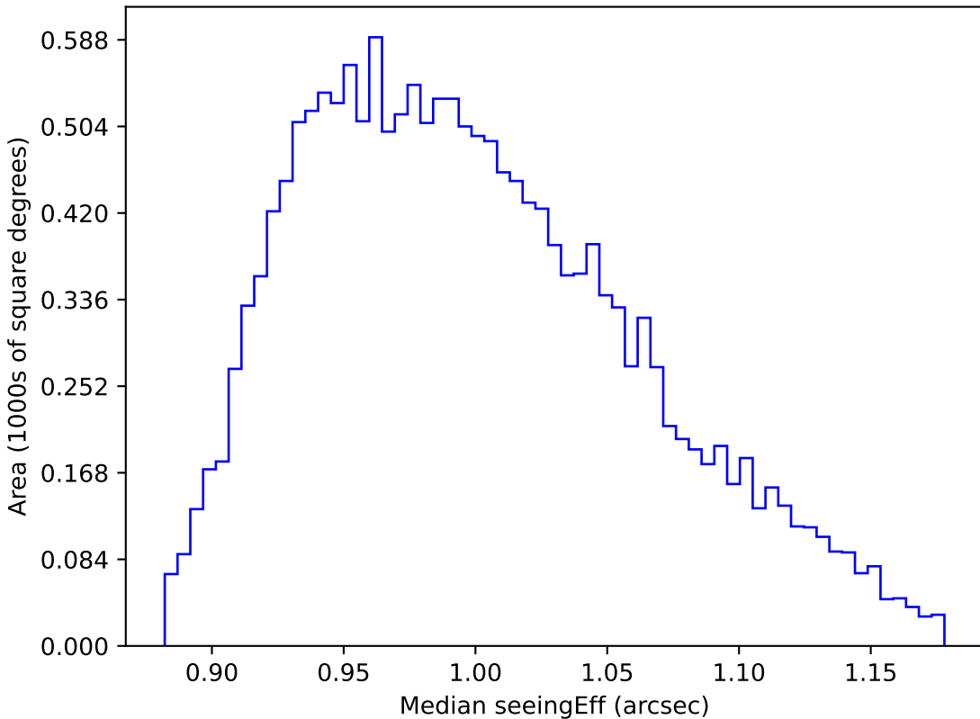
too_100_4v3.4_10yrs WFD y band: Median seeingEff
