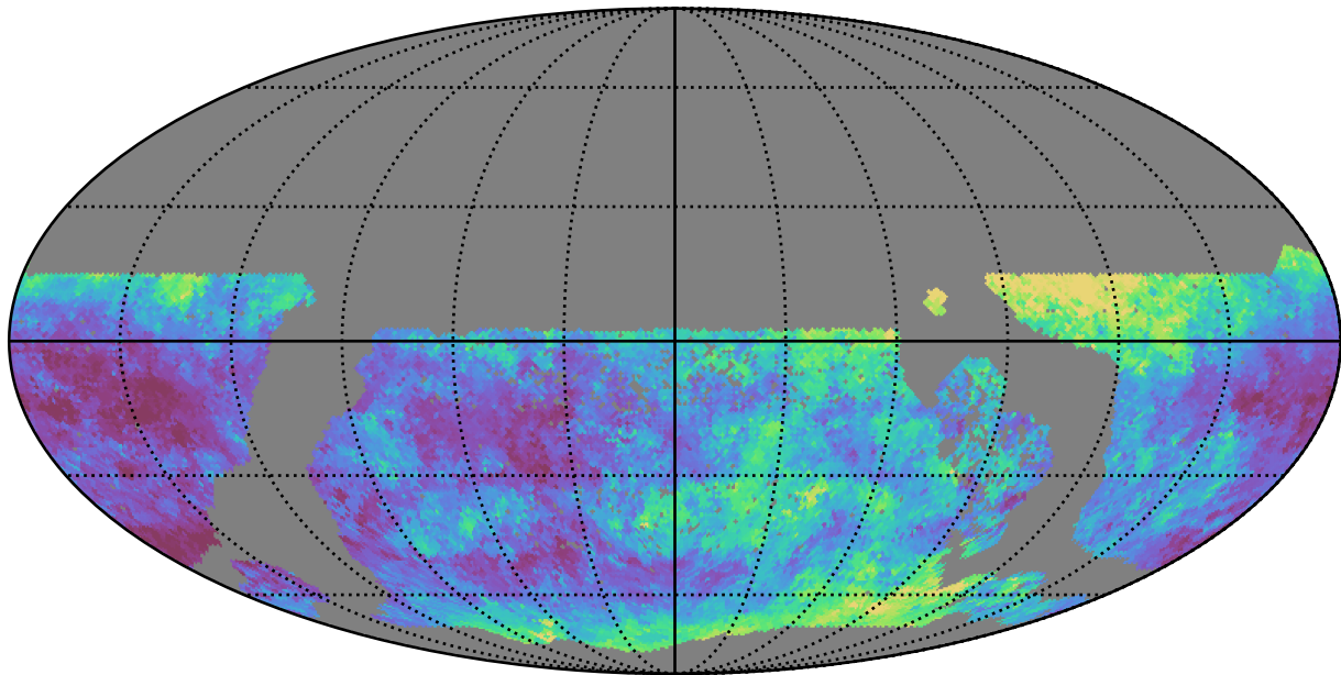
too_100_4v3.4_10yrs WFD u band: Median seeingEff
