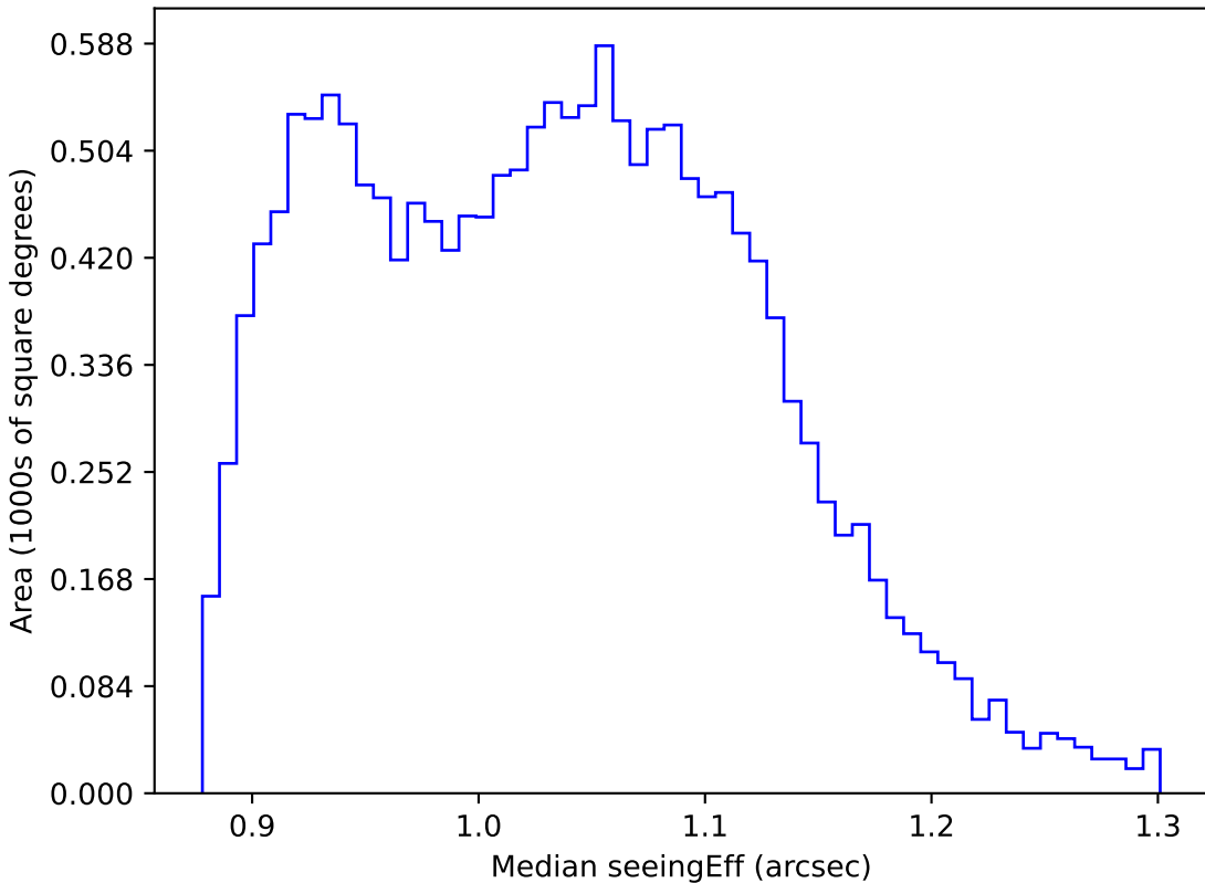
too_100_4v3.4_10yrs WFD r band: Median seeingEff
