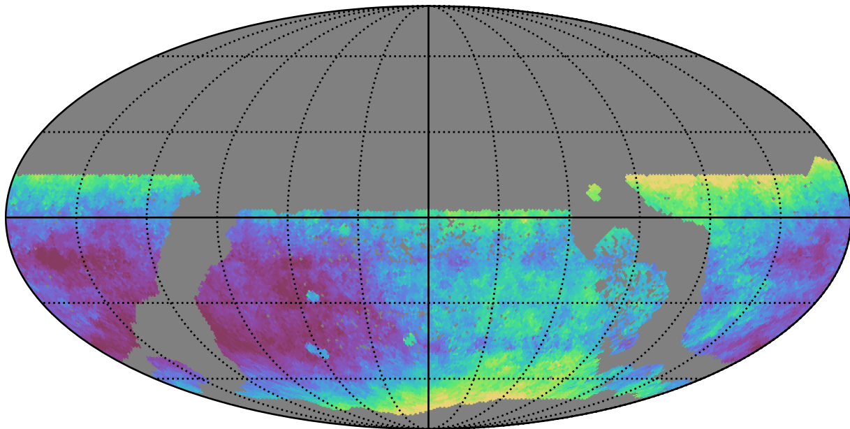
too_100_4v3.4_10yrs WFD i band: Median seeingEff
