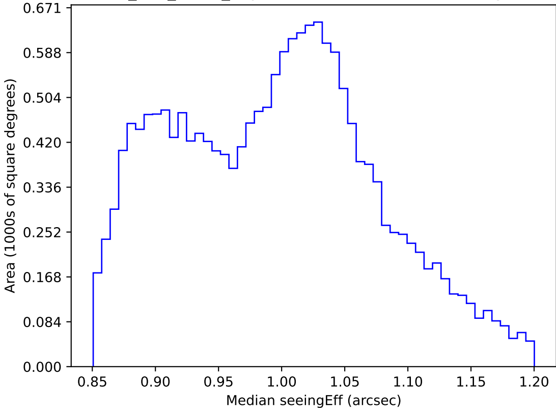
too_100_4v3.4_10yrs WFD i band: Median seeingEff
