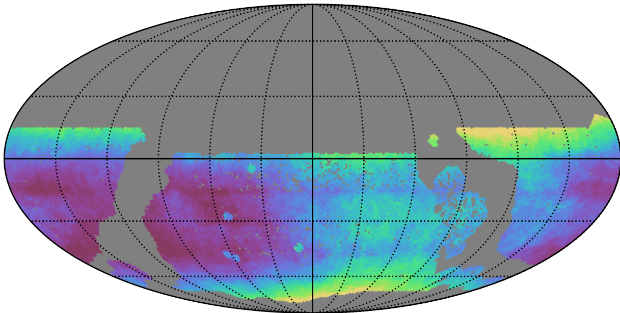
too_100_4v3.4_10yrs WFD all bands: Median seeingEff
