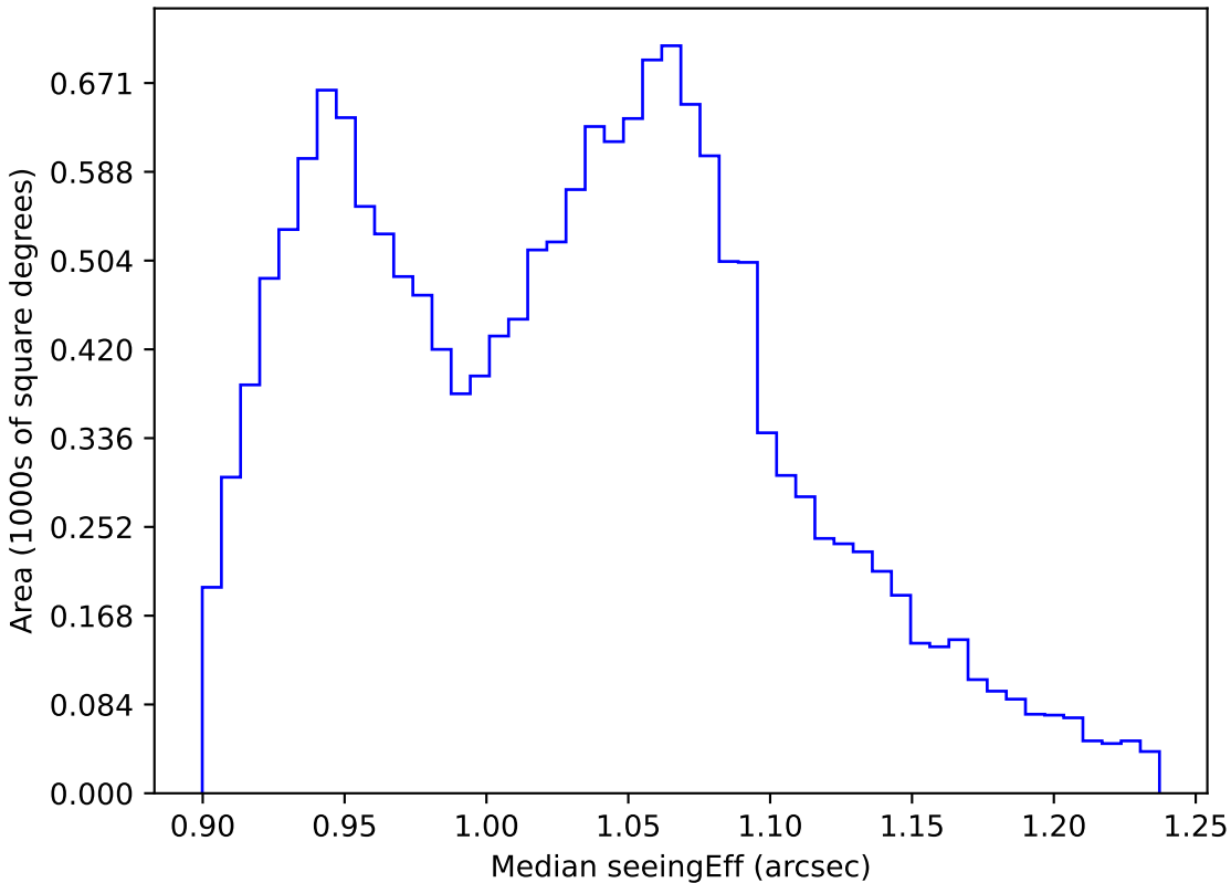
too_100_4v3.4_10yrs WFD all bands: Median seeingEff
