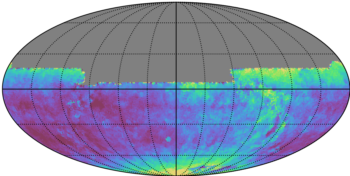
too_100_4v3.4_10yrs All sky y band: Median seeingEff
