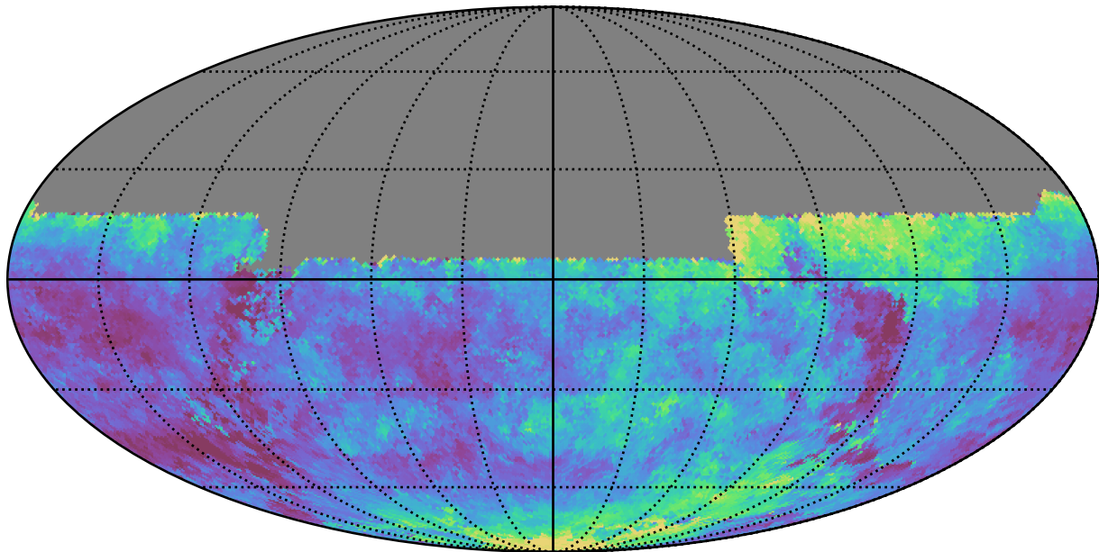
too_100_4v3.4_10yrs All sky u band: Median seeingEff
