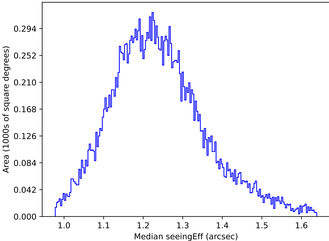
too_100_4v3.4_10yrs All sky u band: Median seeingEff
