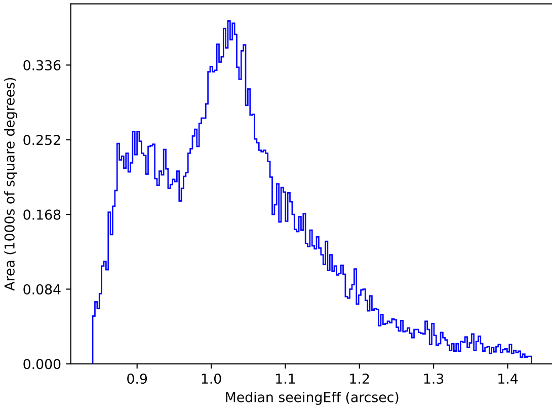
too_100_4v3.4_10yrs All sky i band: Median seeingEff
