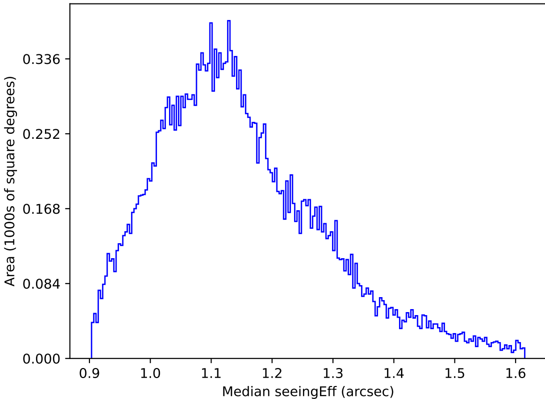
too_100_4v3.4_10yrs All sky g band: Median seeingEff
