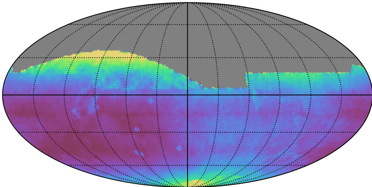
too_100_4v3.4_10yrs All sky all bands: Median seeingEff
