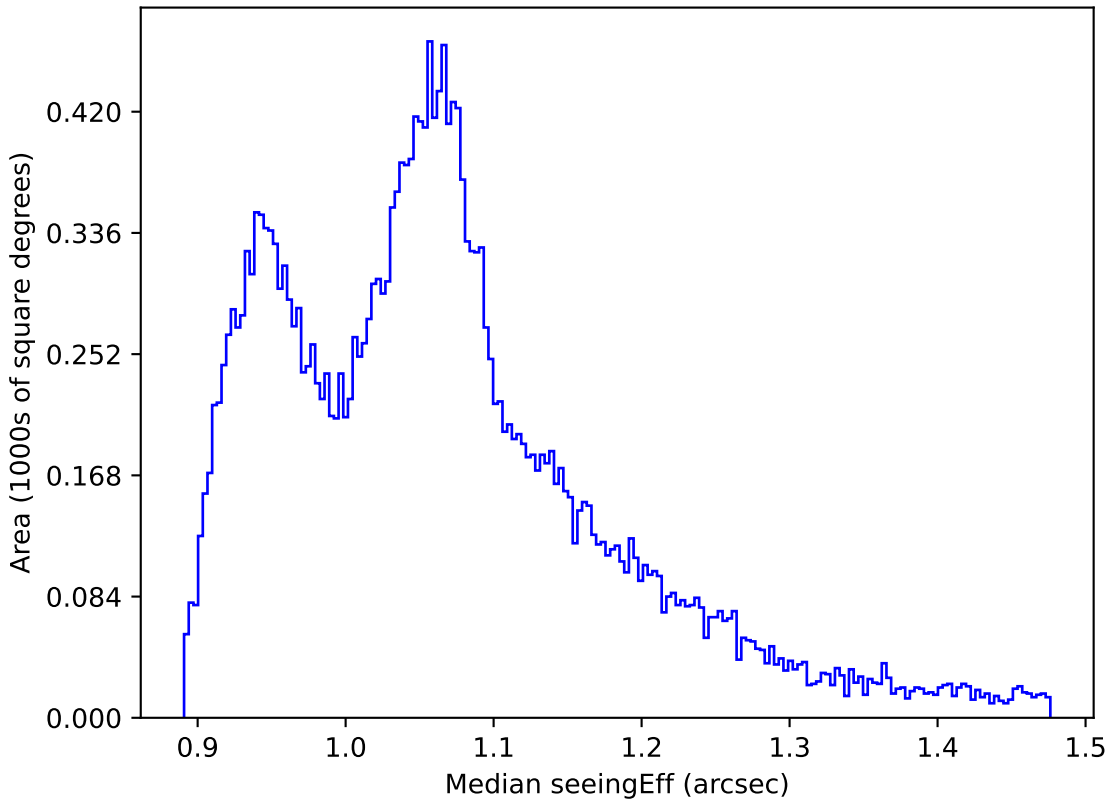
too_100_4v3.4_10yrs All sky all bands: Median seeingEff
