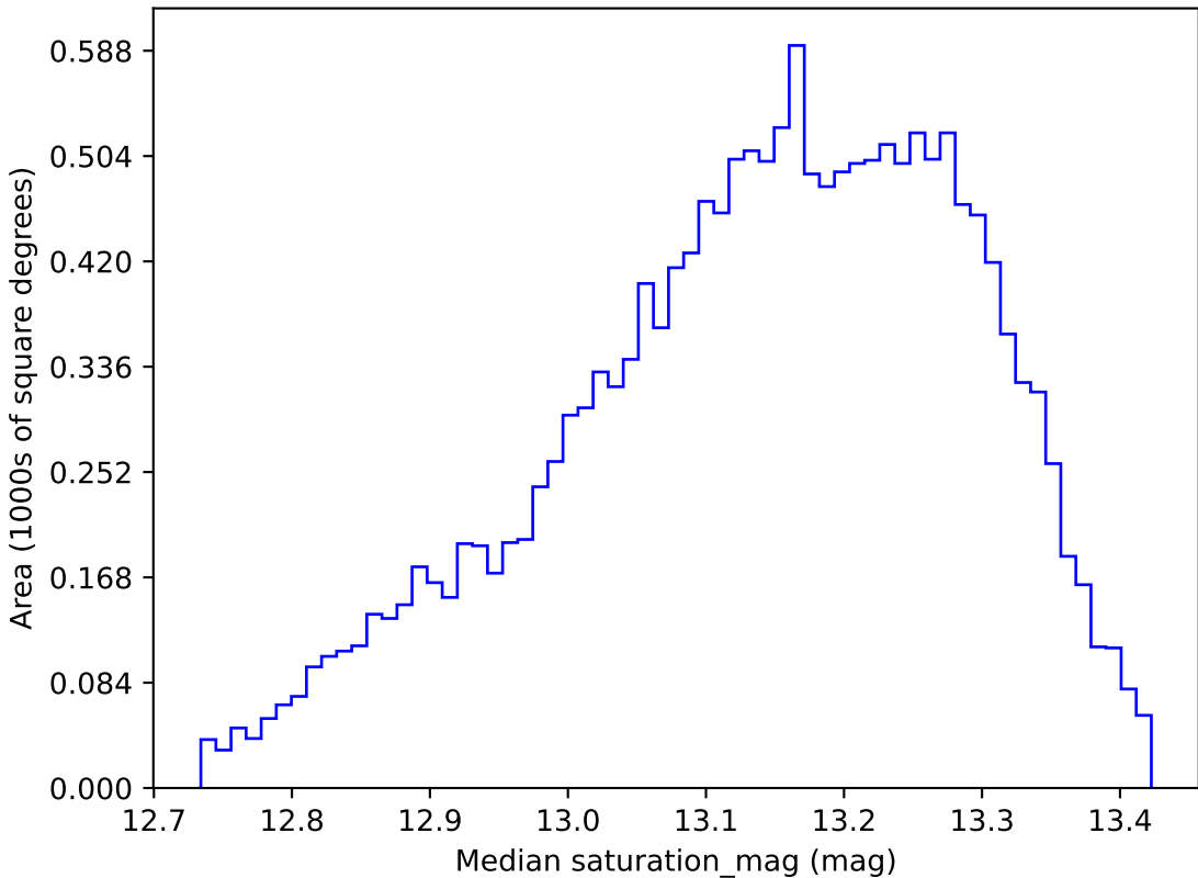
too_100_4v3.4_10yrs WFD y band: Median saturation_mag
