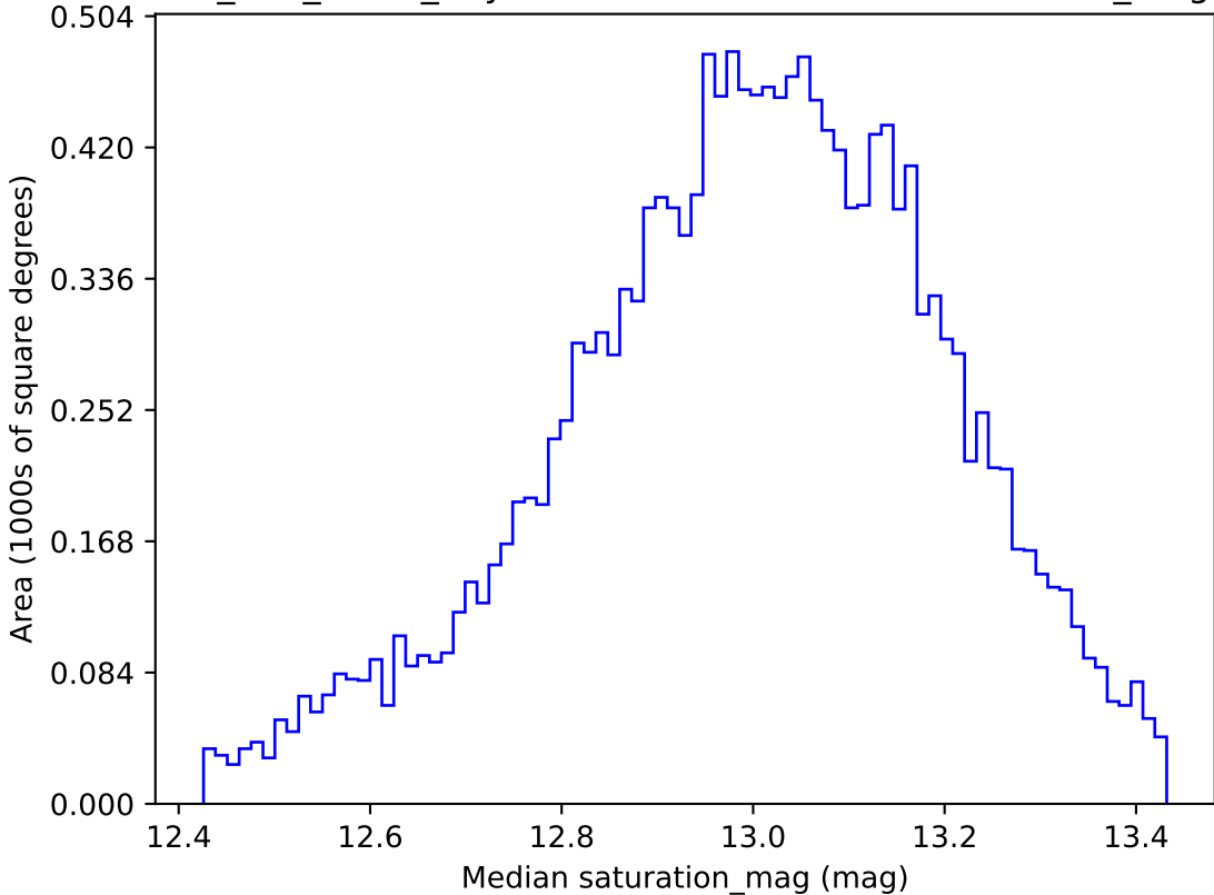
too_100_4v3.4_10yrs WFD u band: Median saturation_mag
