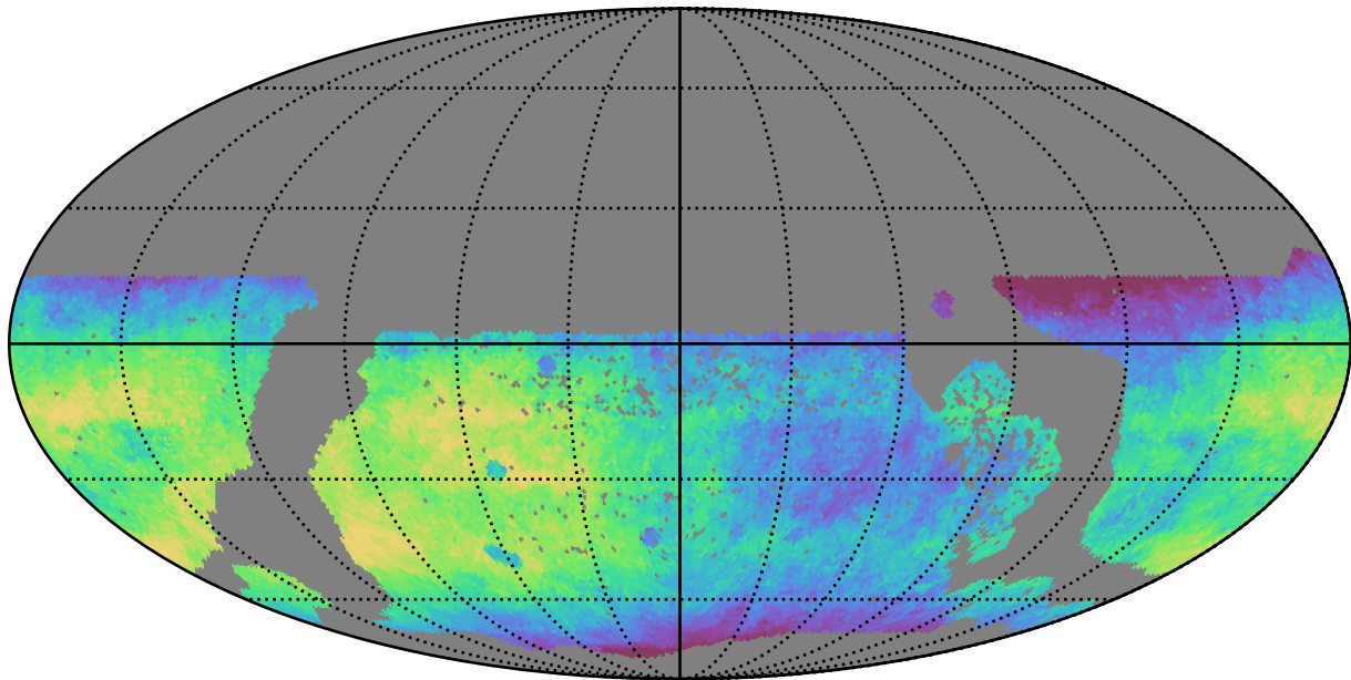
too_100_4v3.4_10yrs WFD r band: Median saturation_mag
