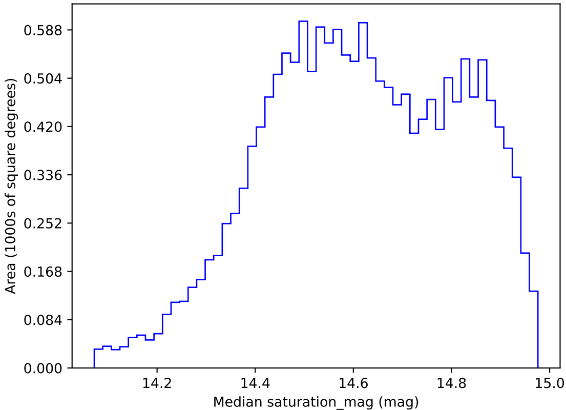
too_100_4v3.4_10yrs WFD r band: Median saturation_mag
