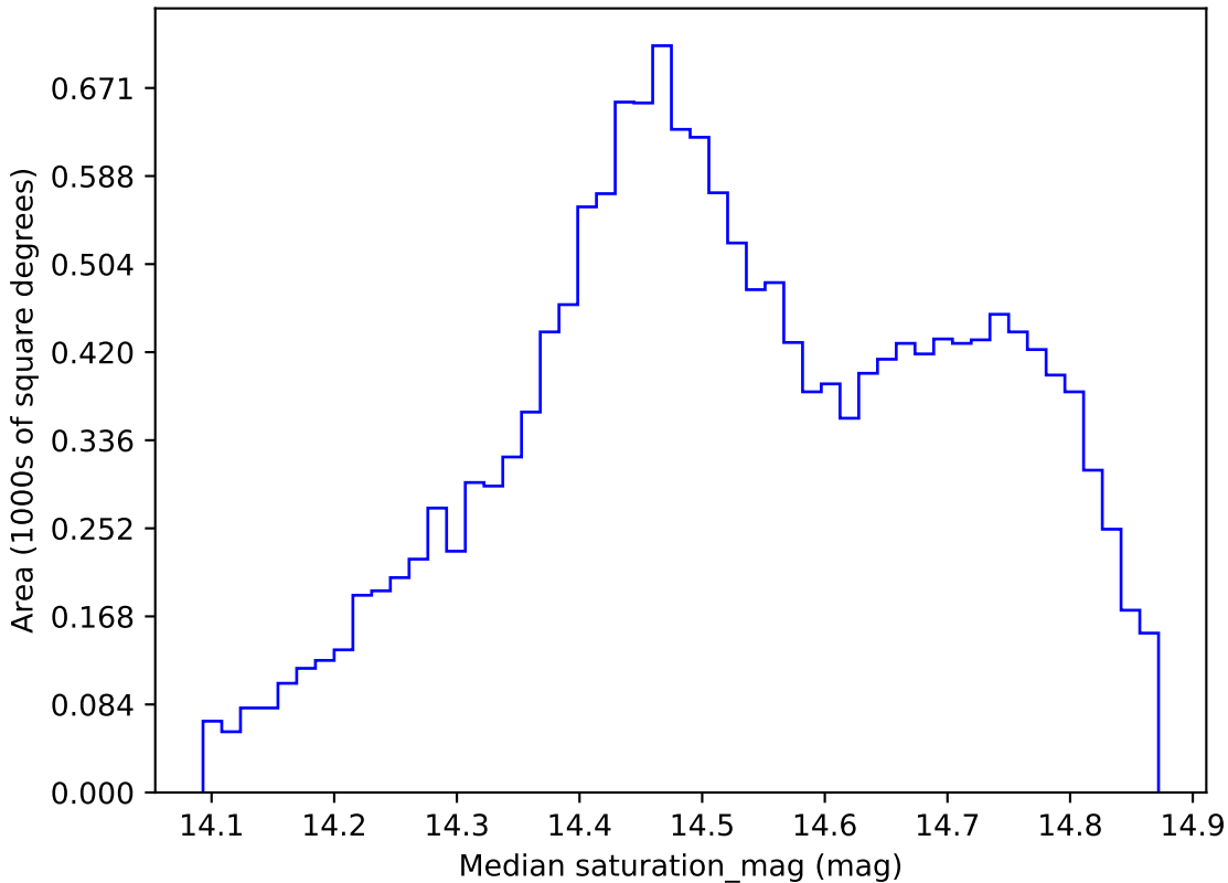
too_100_4v3.4_10yrs WFD i band: Median saturation_mag
