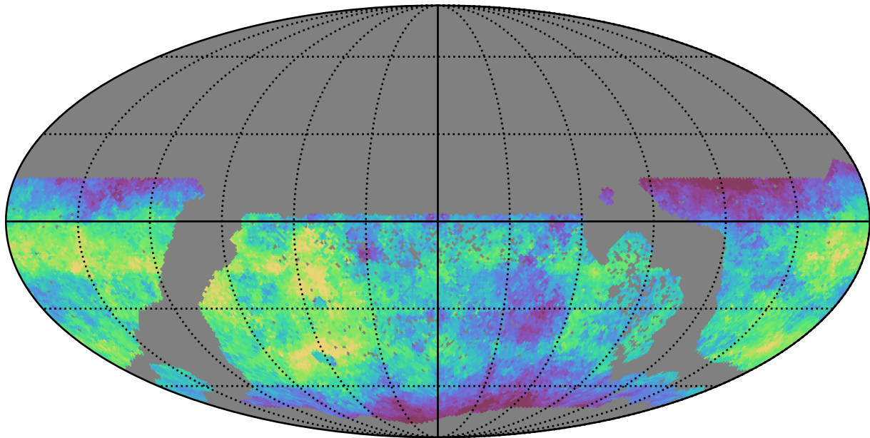
too_100_4v3.4_10yrs WFD g band: Median saturation_mag
