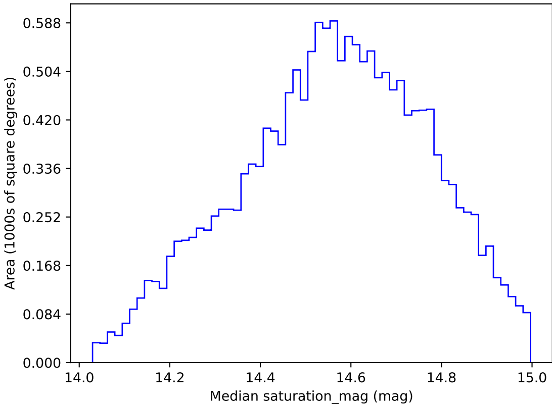
too_100_4v3.4_10yrs WFD g band: Median saturation_mag
