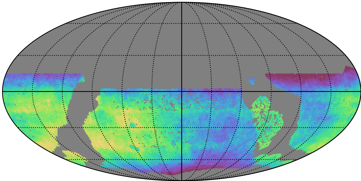
too_100_4v3.4_10yrs WFD all bands: Median saturation_mag
