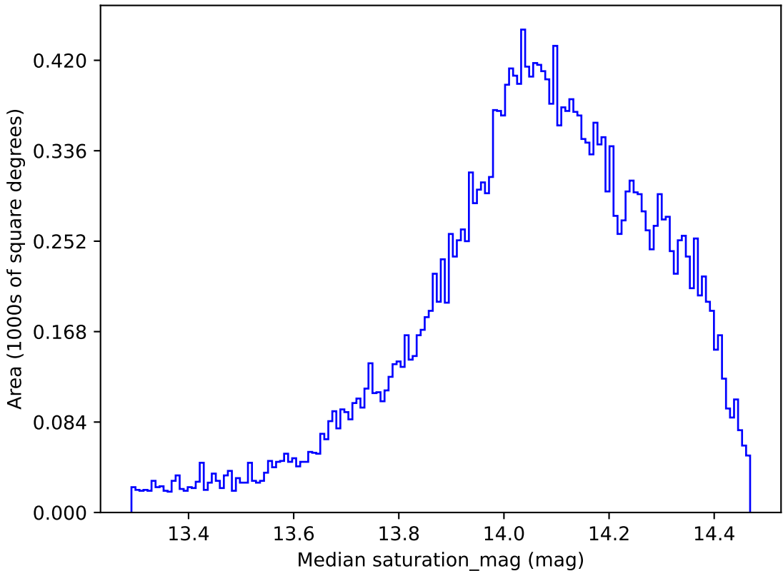
too_100_4v3.4_10yrs All sky z band: Median saturation_mag
