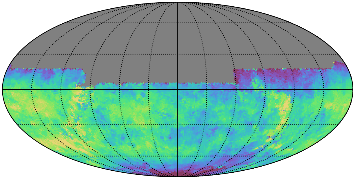
too_100_4v3.4_10yrs All sky u band: Median saturation_mag
